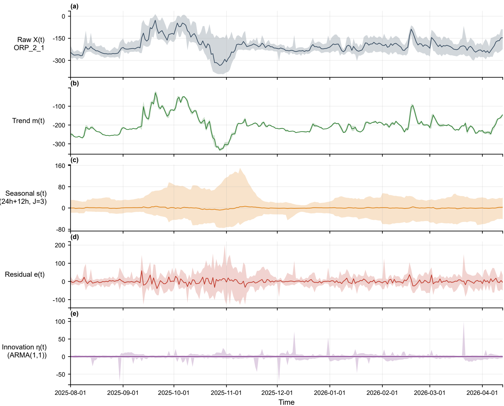
Full-span daily overview — ORP_2_1 (anaerobic, min) [2025-08-01~2026-04-13]
